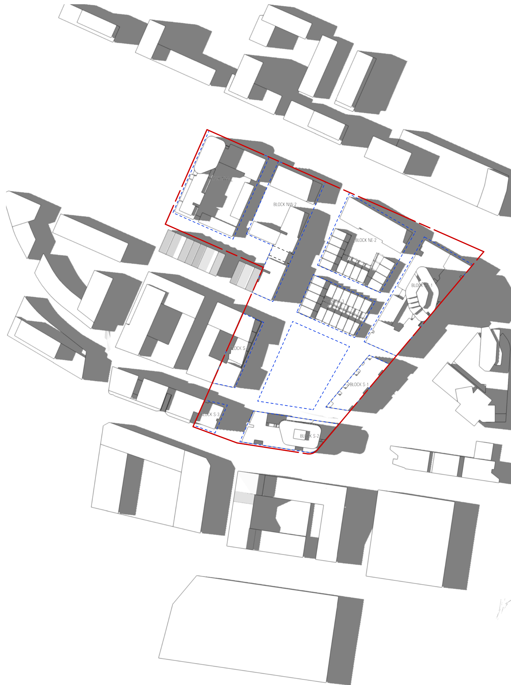
Proposed Envelopes 21/12 1500
